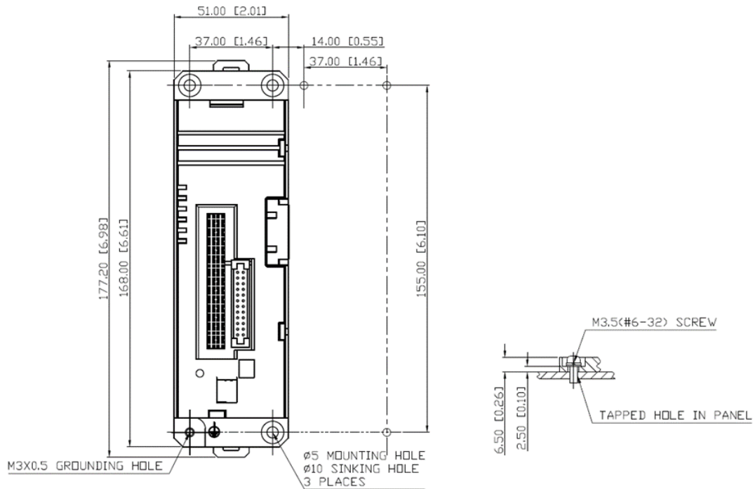
Figure 4: Panel Mounting
