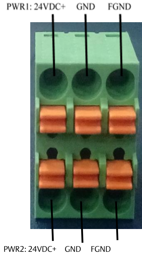
Figure 6: Terminal Connection
