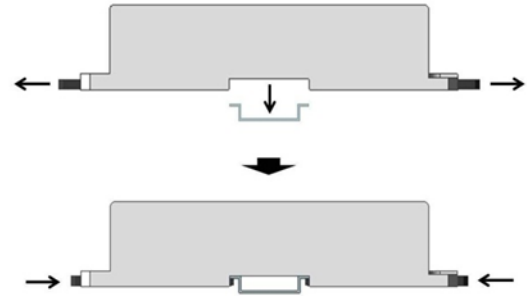
Figure 3: Installing on DIN Rail
