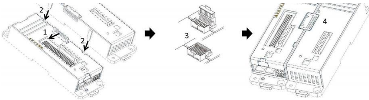
Figure 2: Connecting Expansion Carrier
