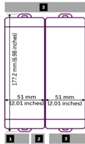
Figure 1: Dimension
