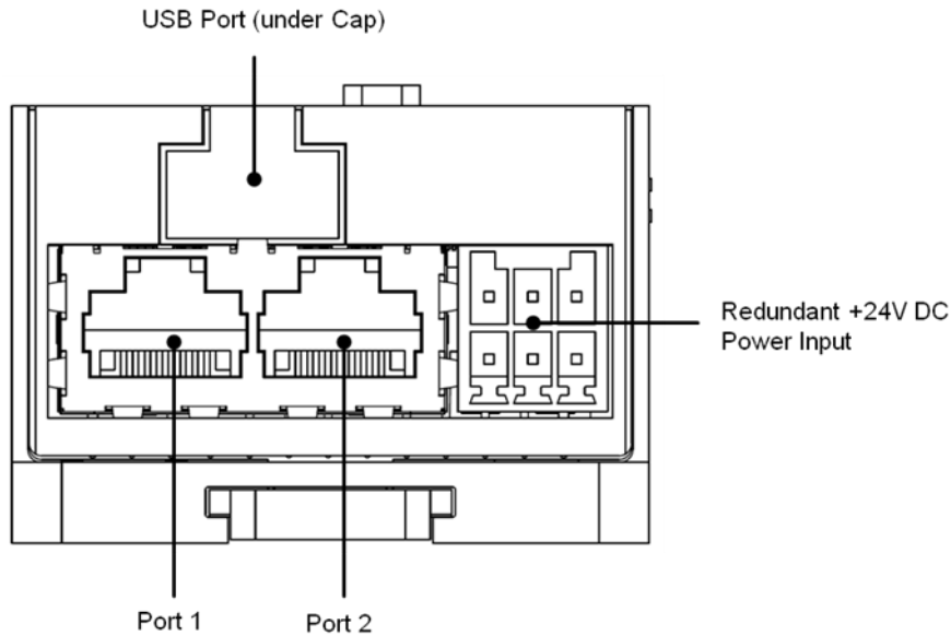
Figure 7: Profinet Connection
